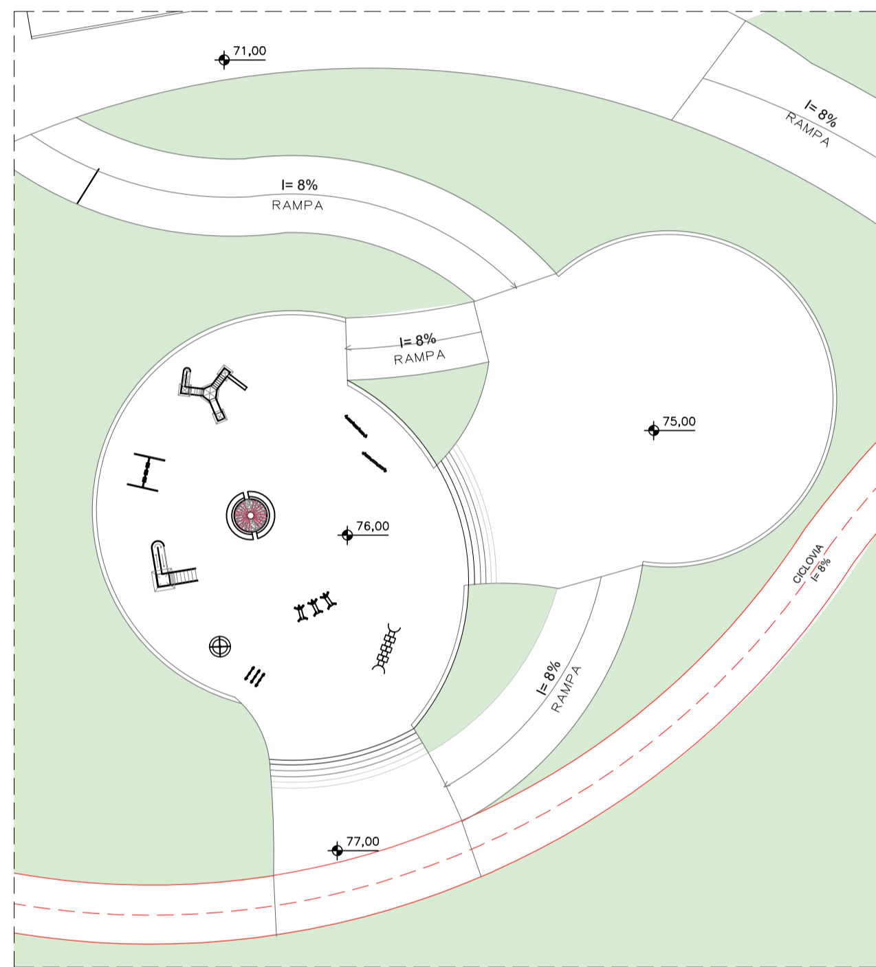
DETALHE PLAY GROUND ESC 1/500
